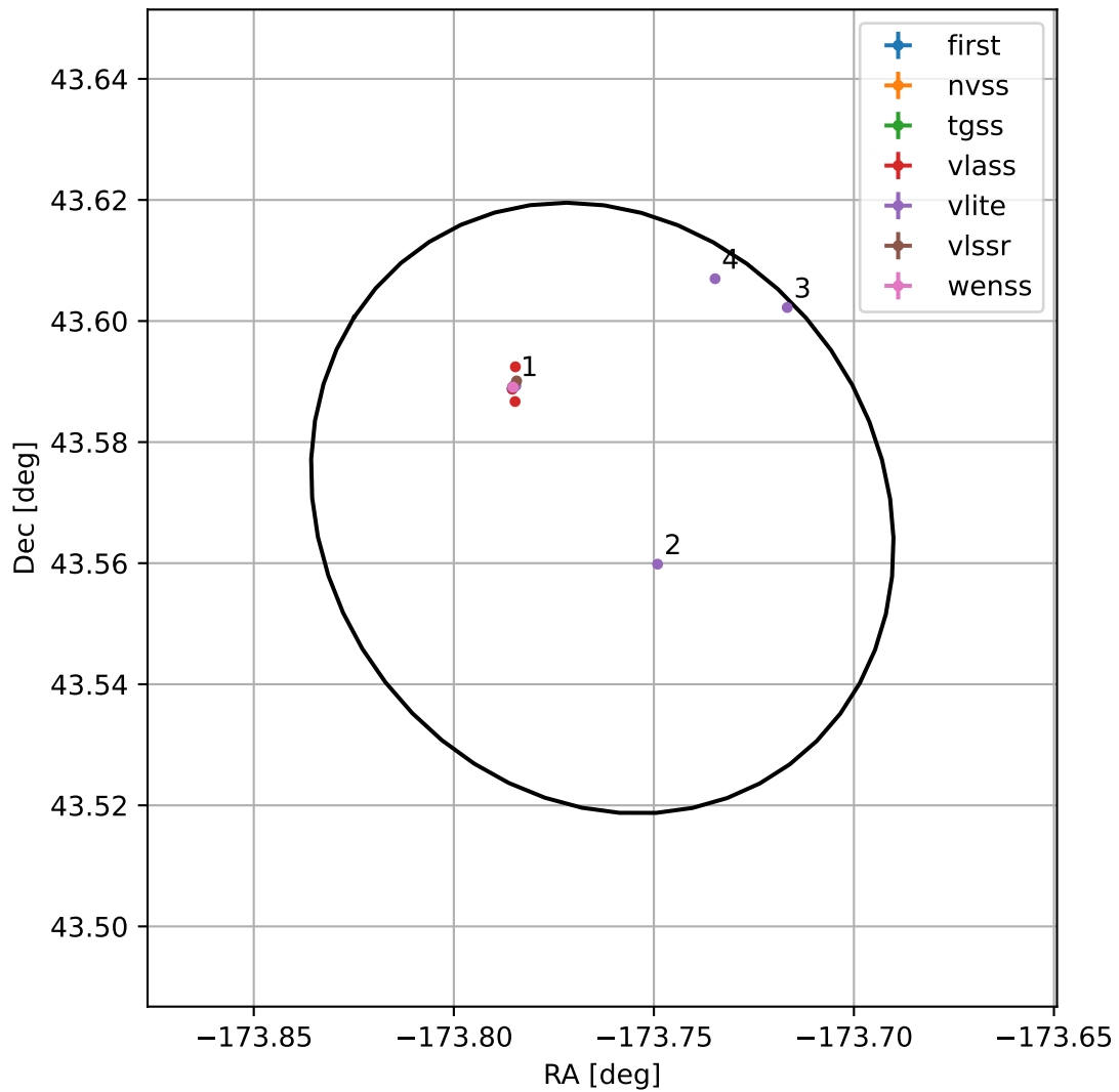
4FGL J1224.9+4334
