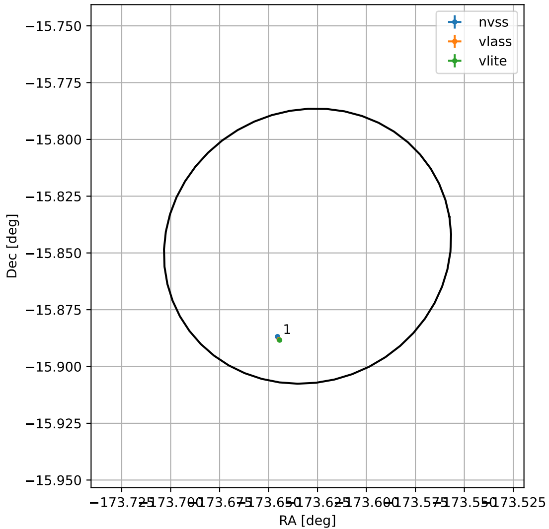
4FGL J1225.4-1550
