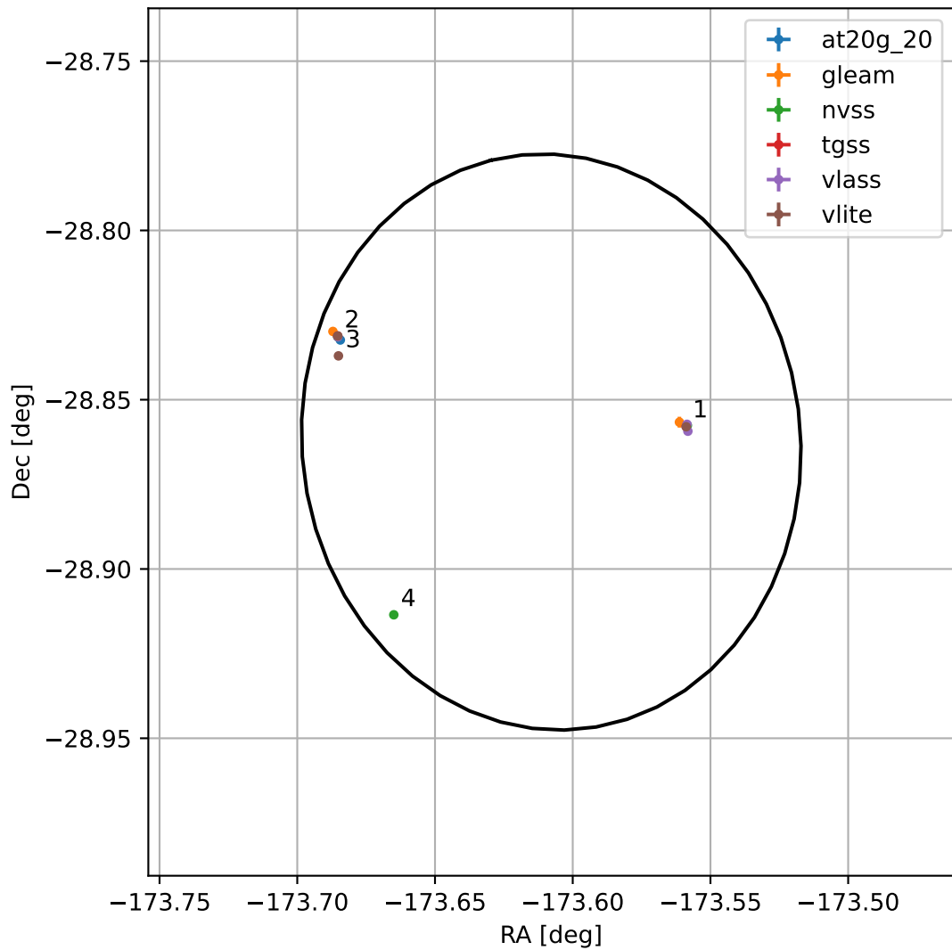
4FGL J1225.5-2851
