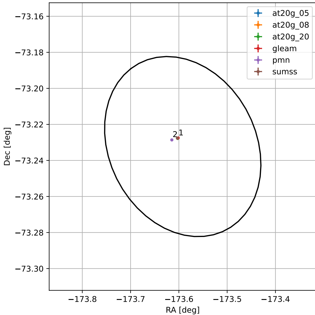
4FGL J1225.6-7313
