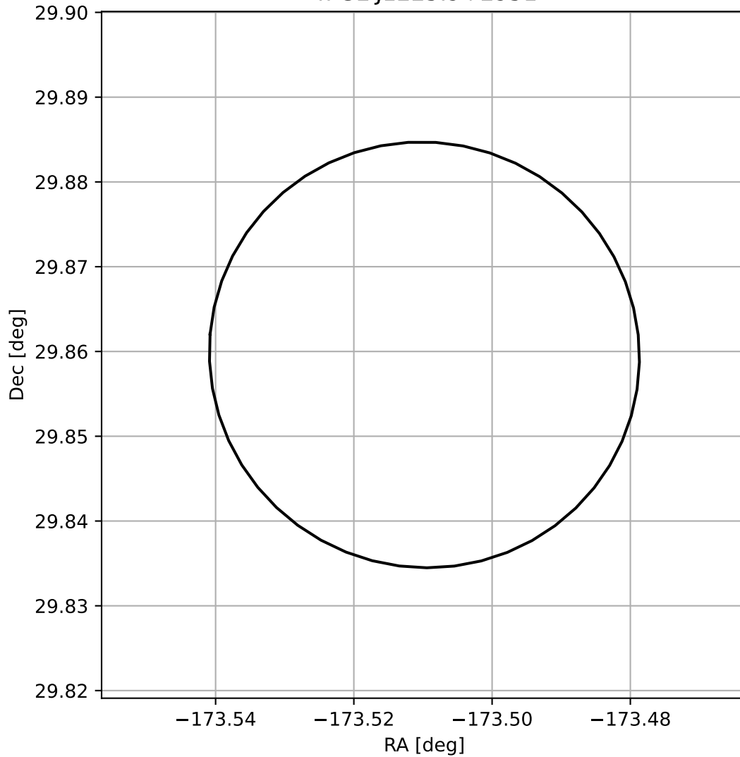
4FGL J1225.9+2951
