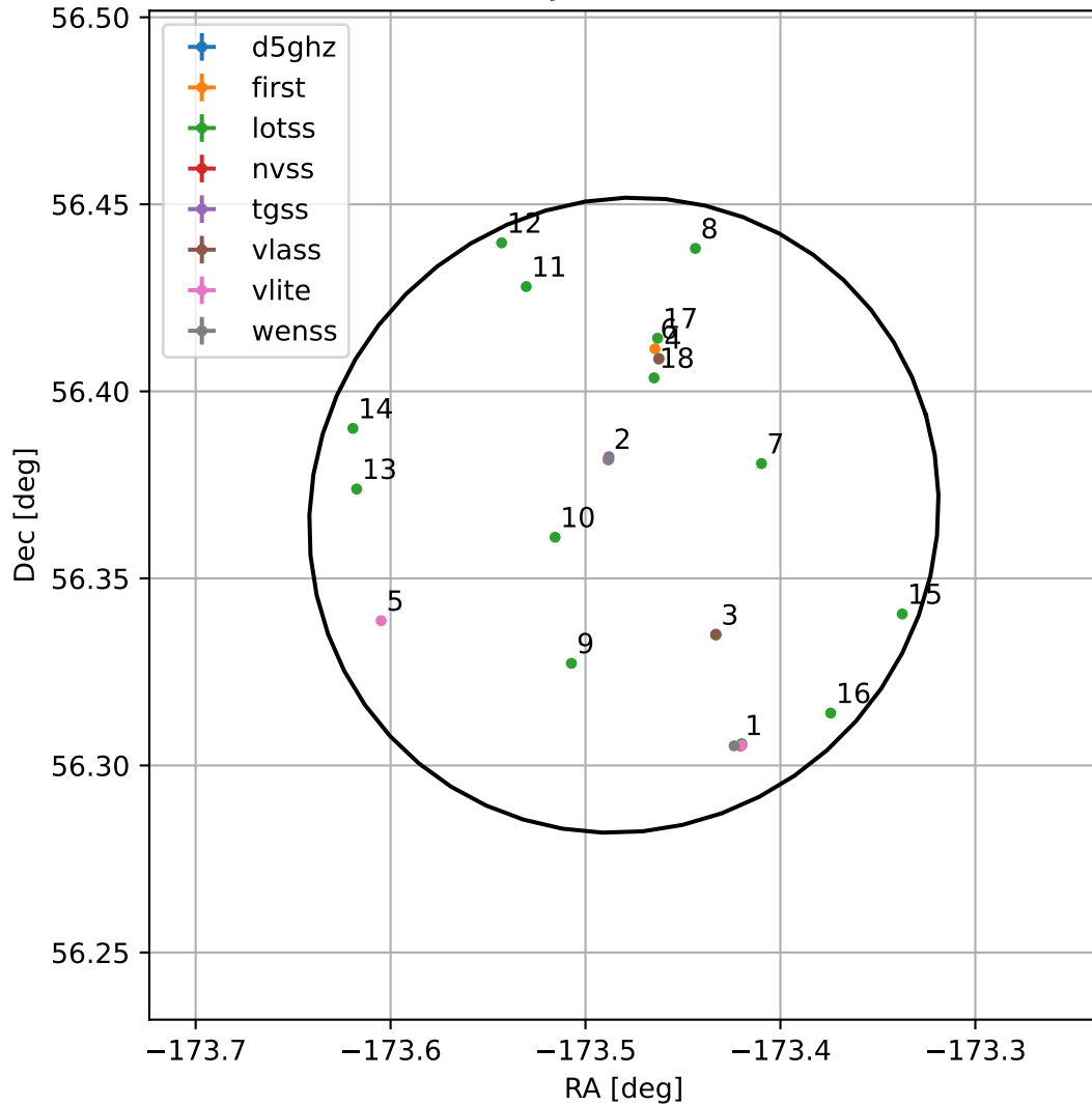
4FGL J1226.0+5622
