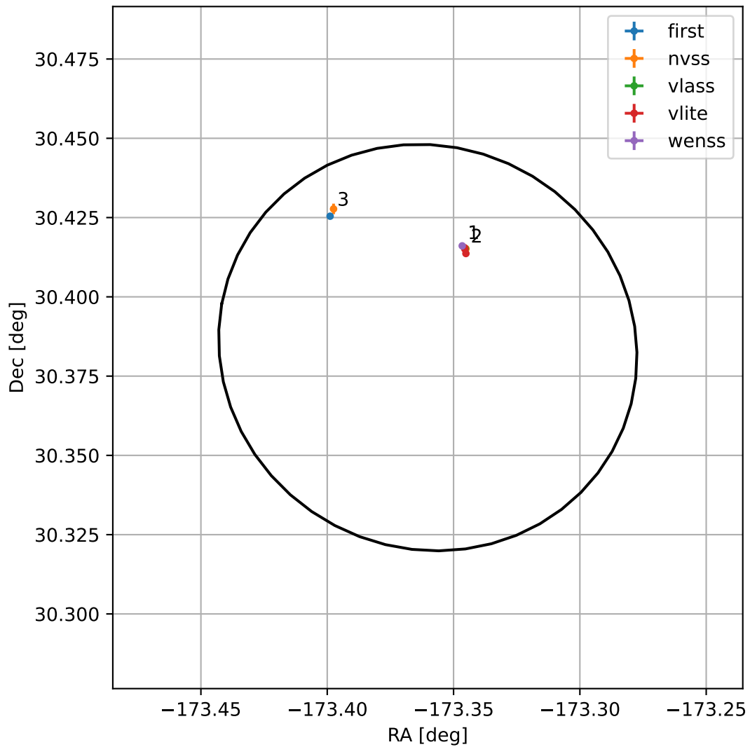
4FGL J1226.5+3023
