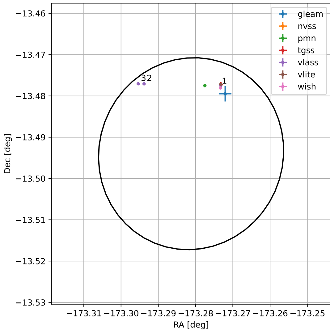
4FGL J1226.8-1329
