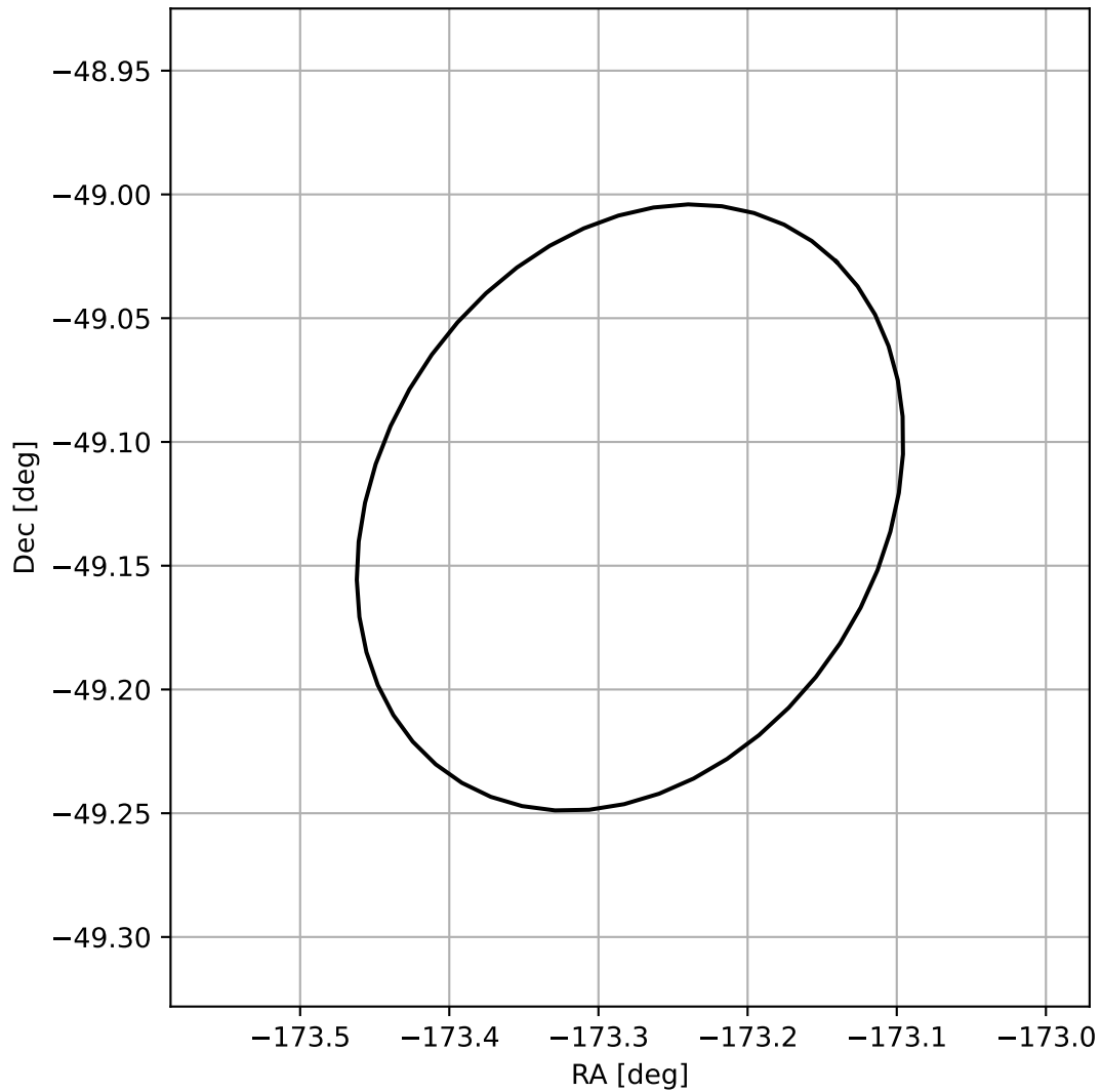
4FGL J1226.8-4907
