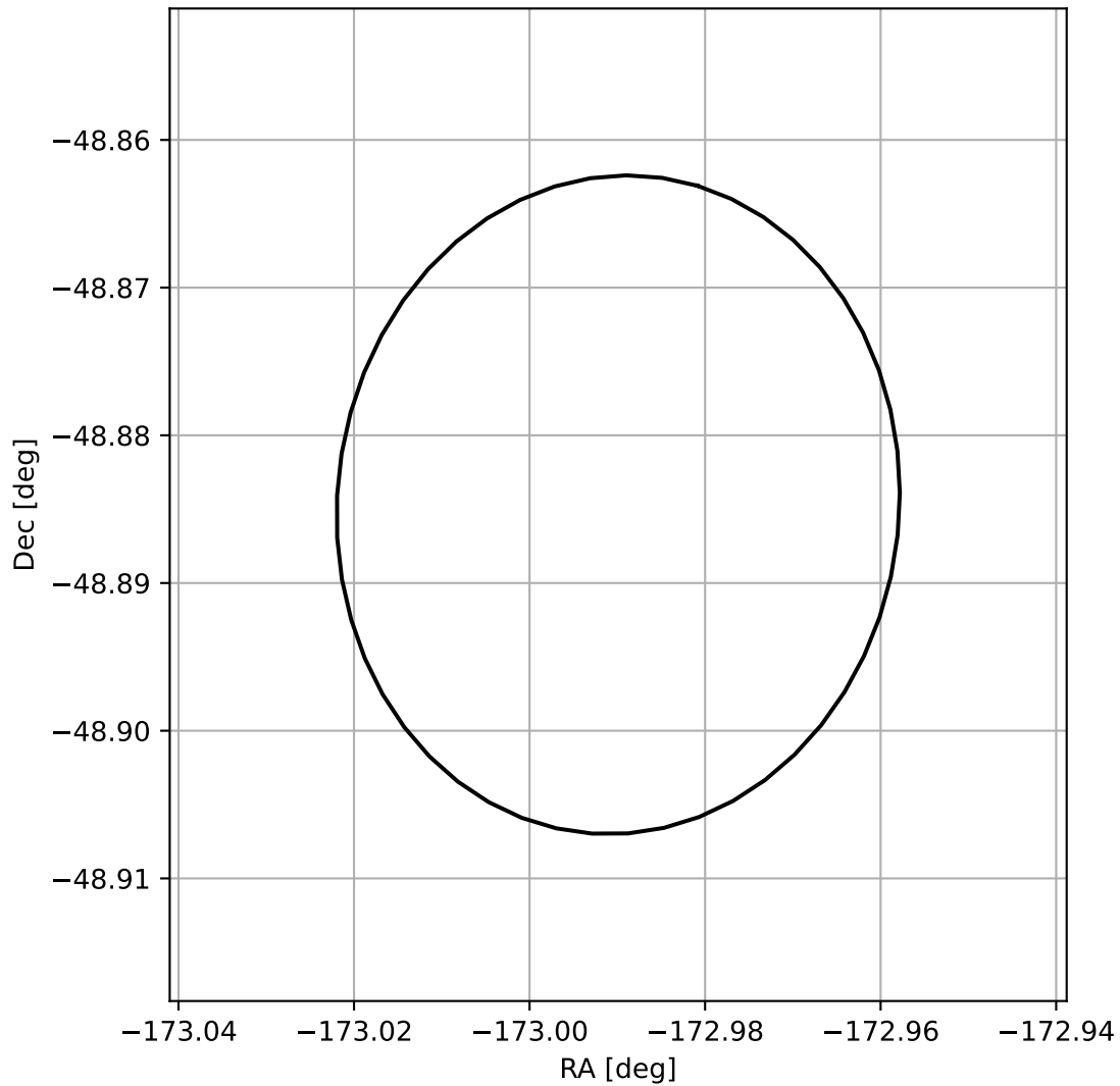
4FGL J1228.0-4853
