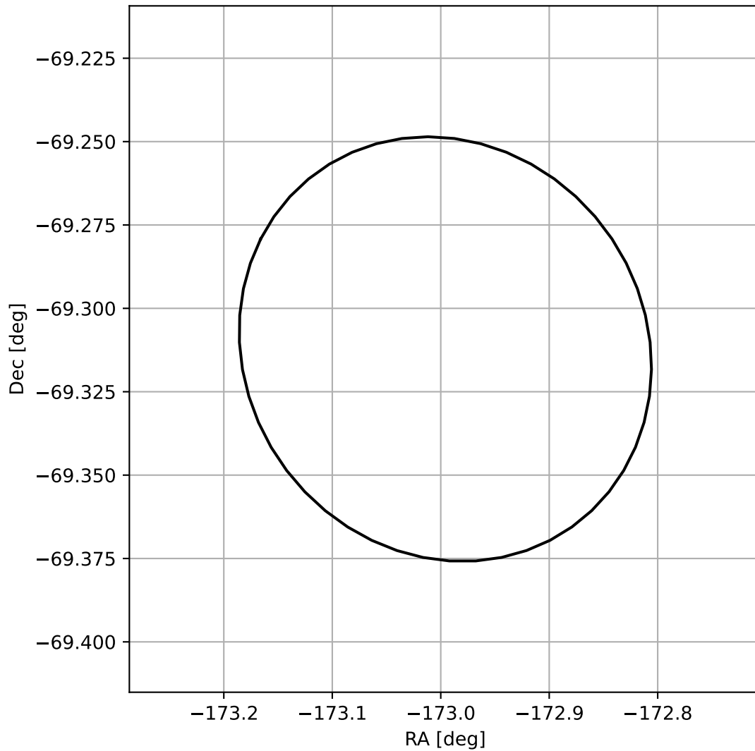
4FGL J1228.0-6918
