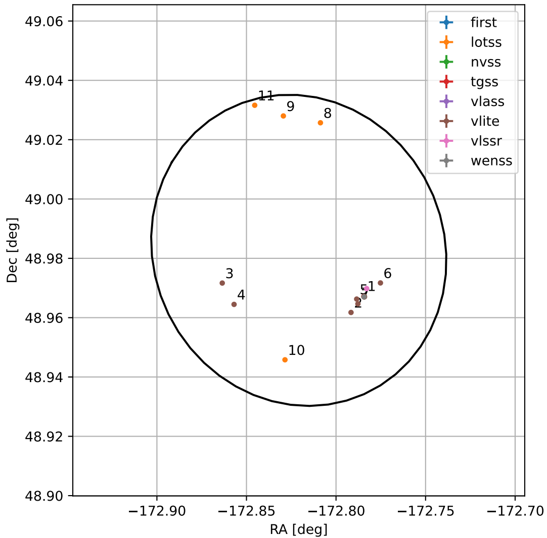
4FGL J1228.7+4858
