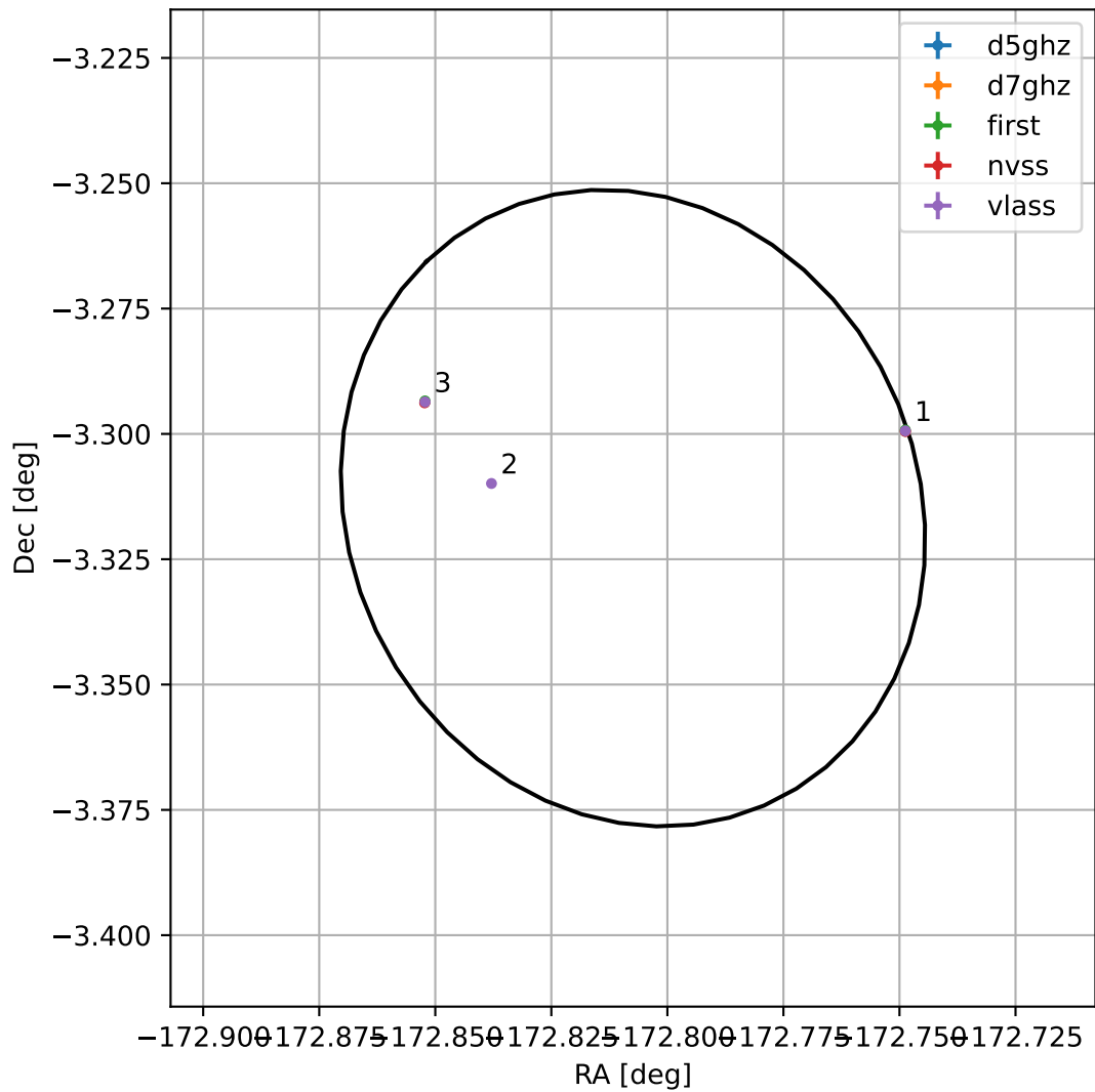
4FGL J1228.7-0318
