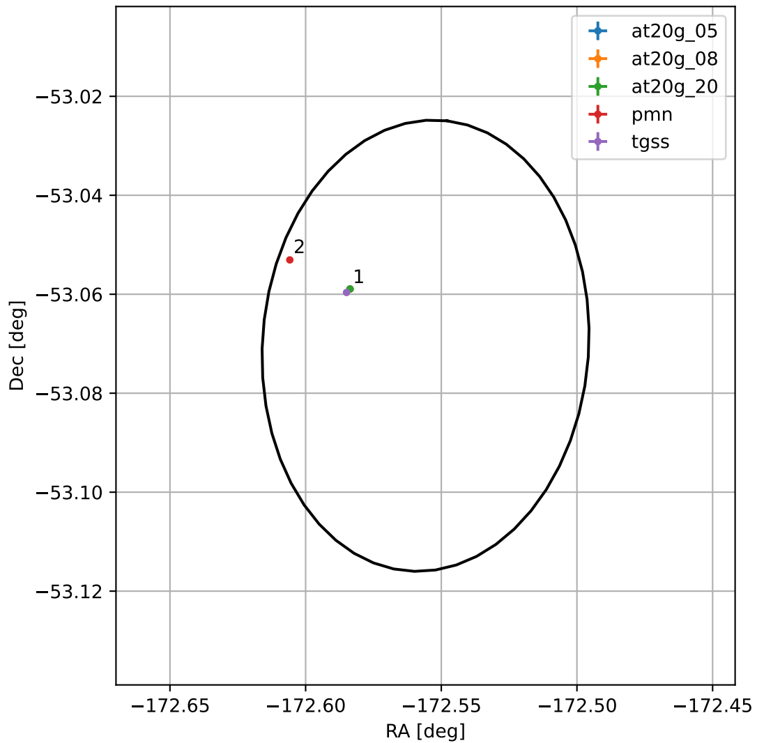
4FGL J1229.7-5304
