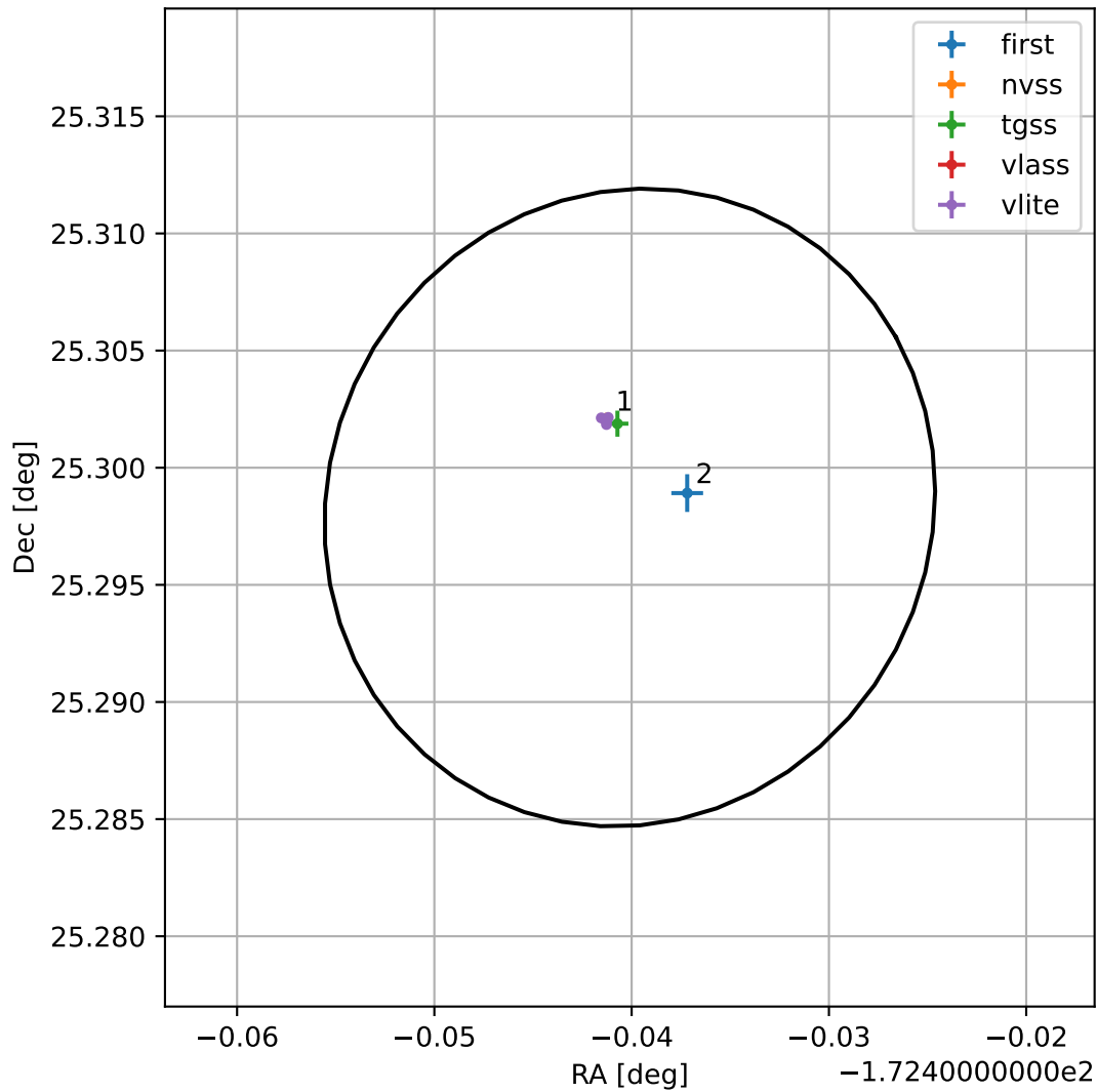
4FGL J1230.2+2517
