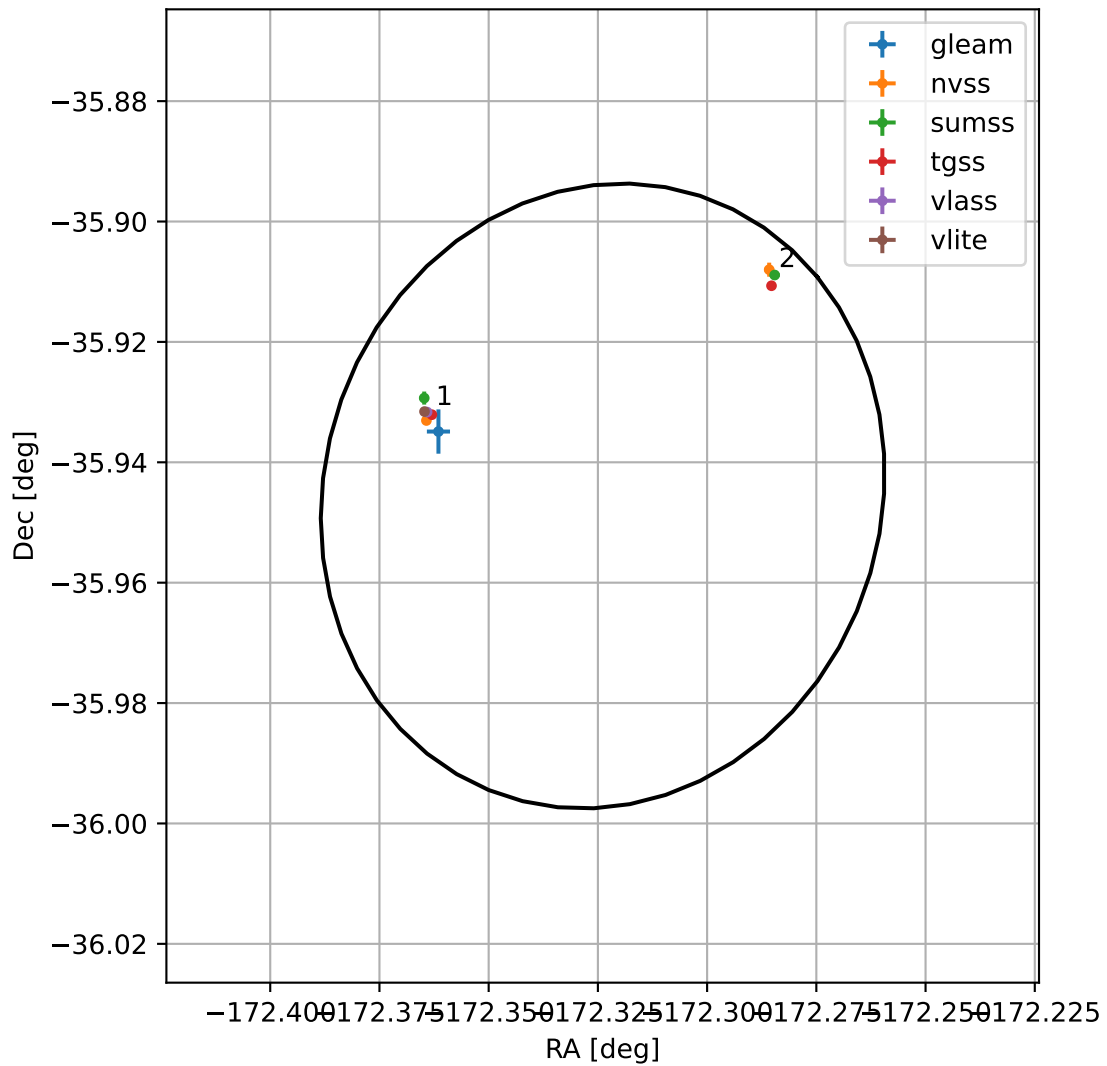
4FGL J1230.7-3556
