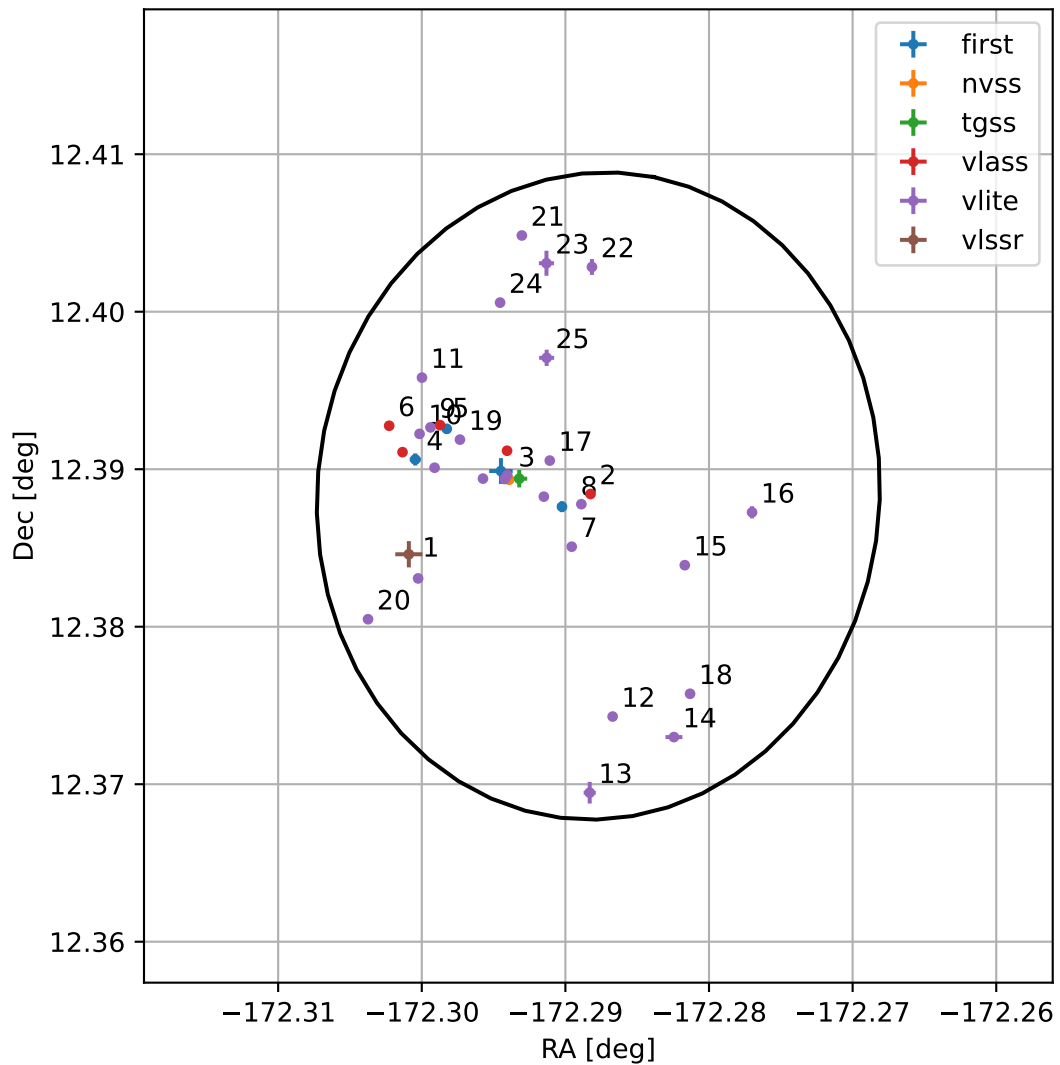
4FGL J1230.8+1223
