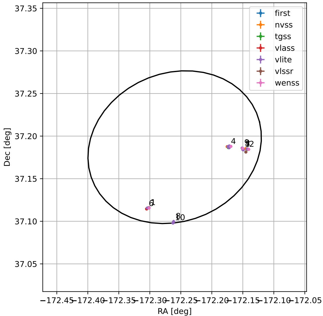
4FGL J1230.9+3711
