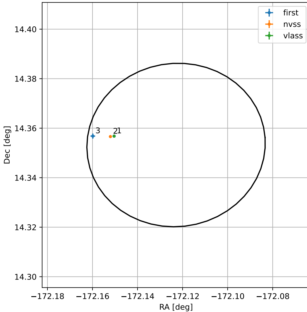
4FGL J1231.5+1421
