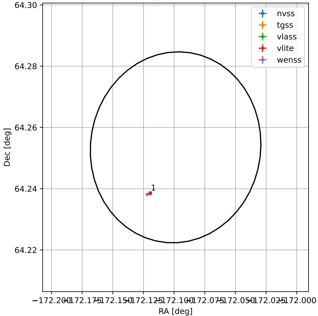
4FGL J1231.6+6415
