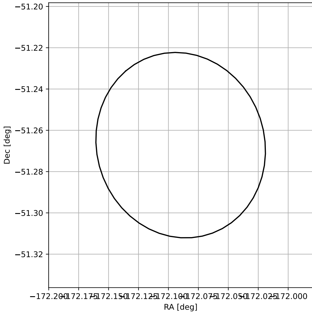
4FGL J1231.6-5116
