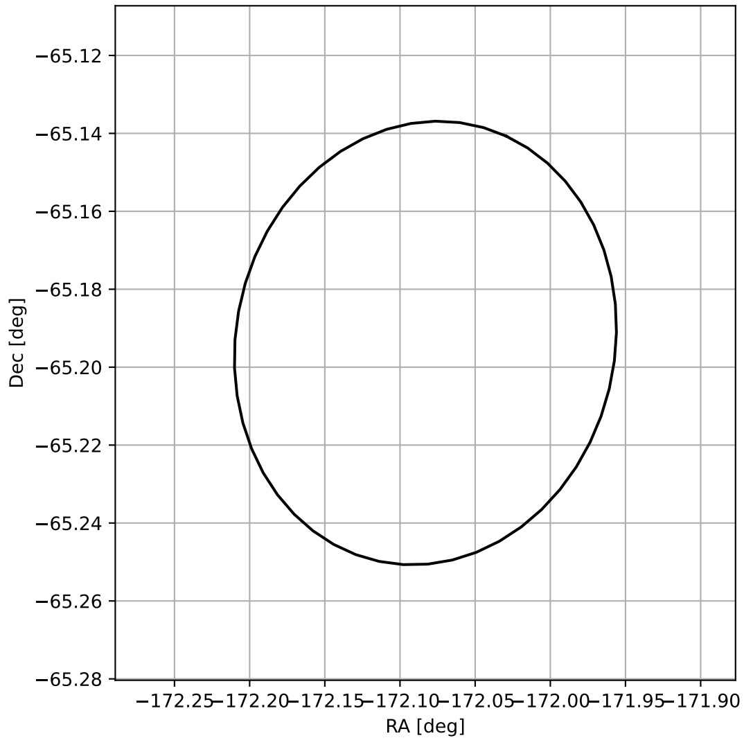
4FGL J1231.6-6511
