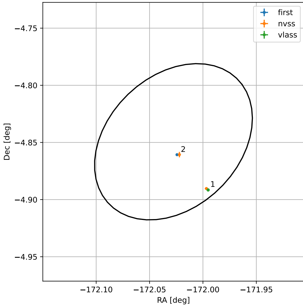
4FGL J1231.8-0450
