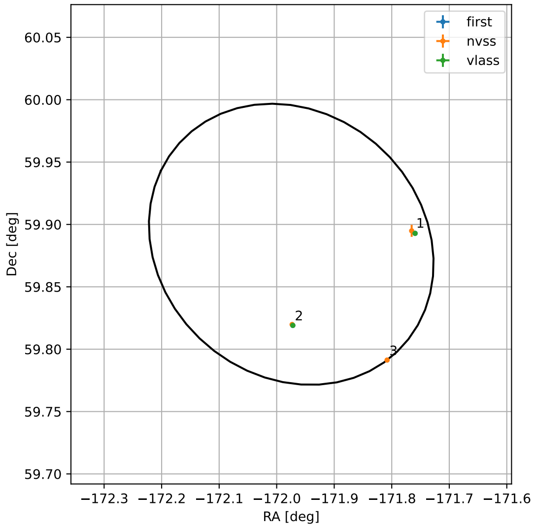
4FGL J1232.1+5953
