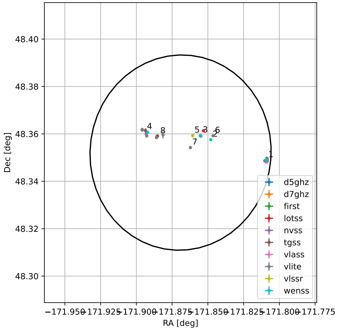
4FGL J1232.5+4821
