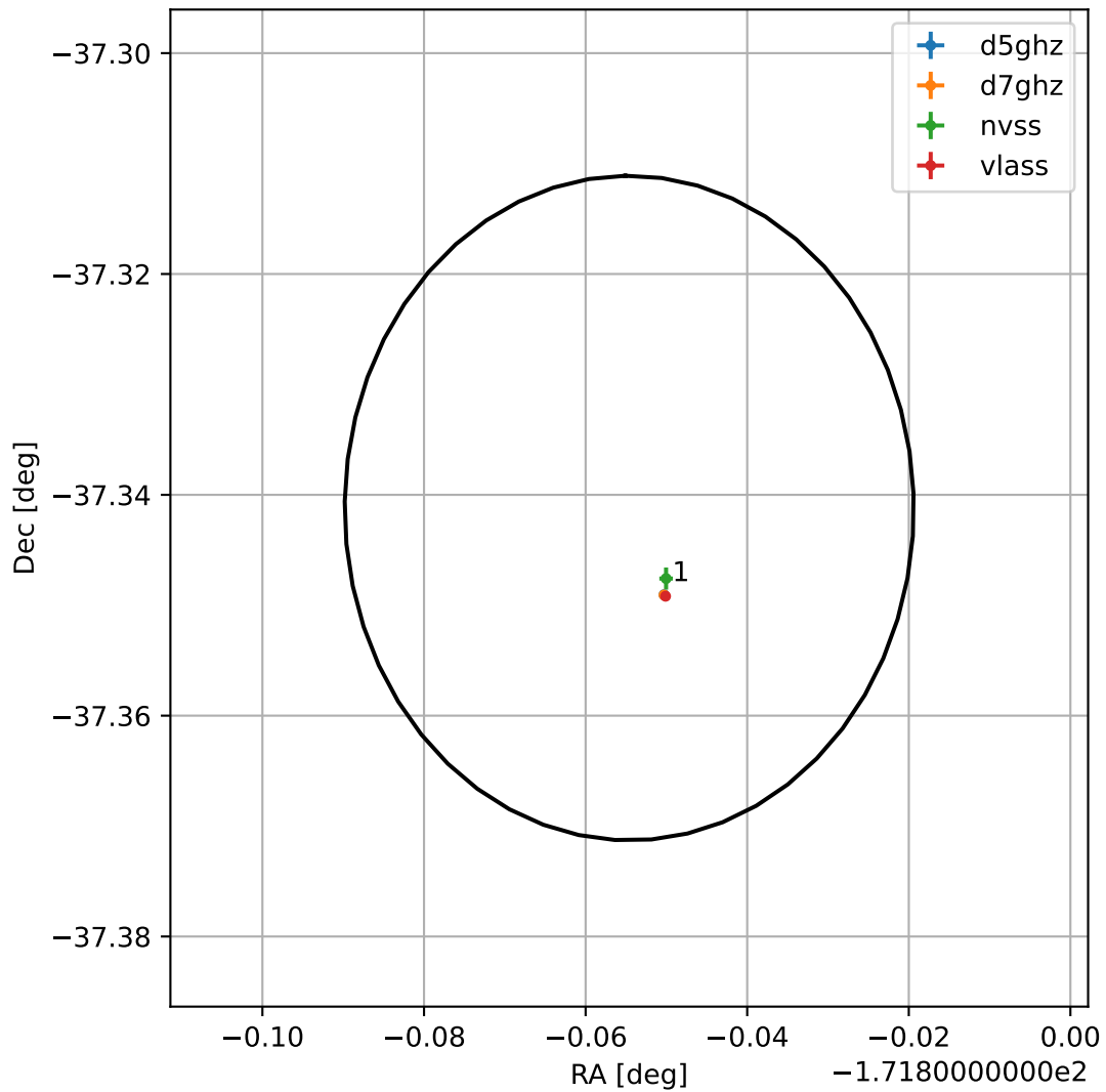
4FGL J1232.5-3720
