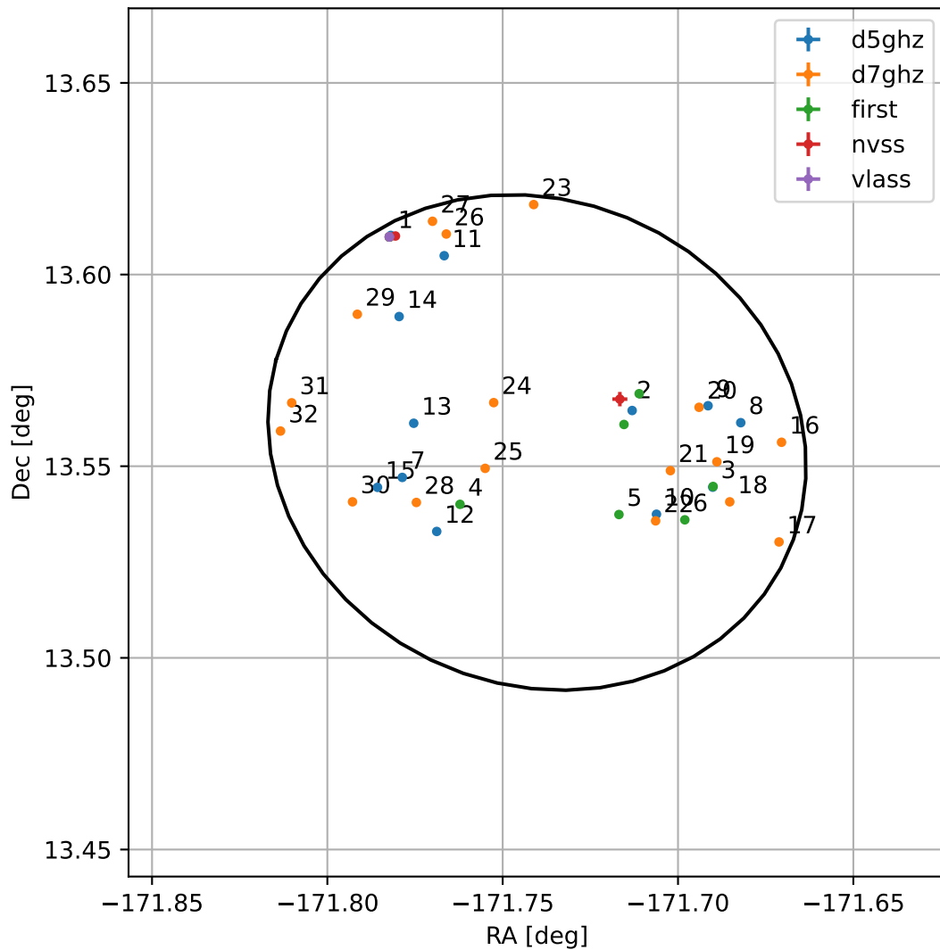
4FGL J1233.0+1333
