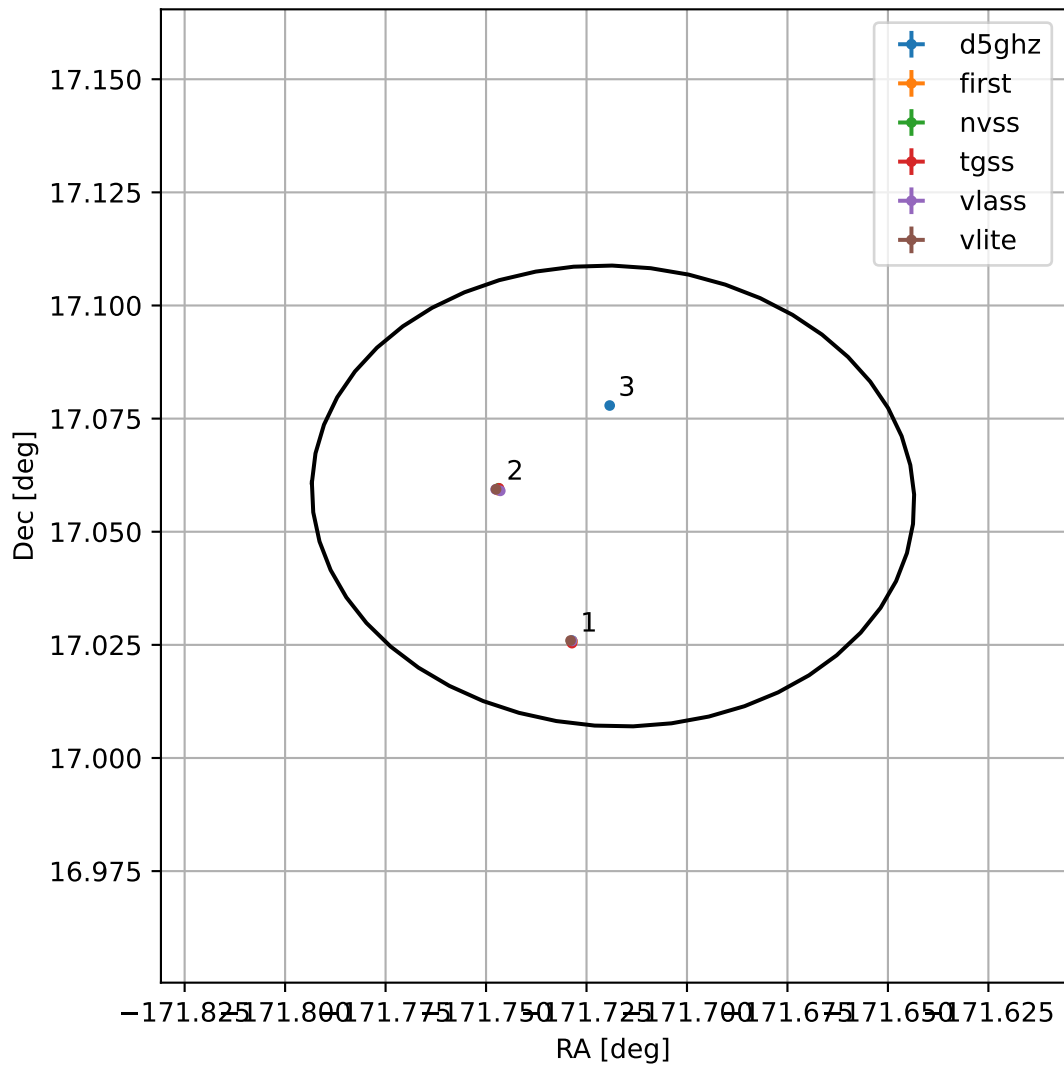
4FGL J1233.1+1703
