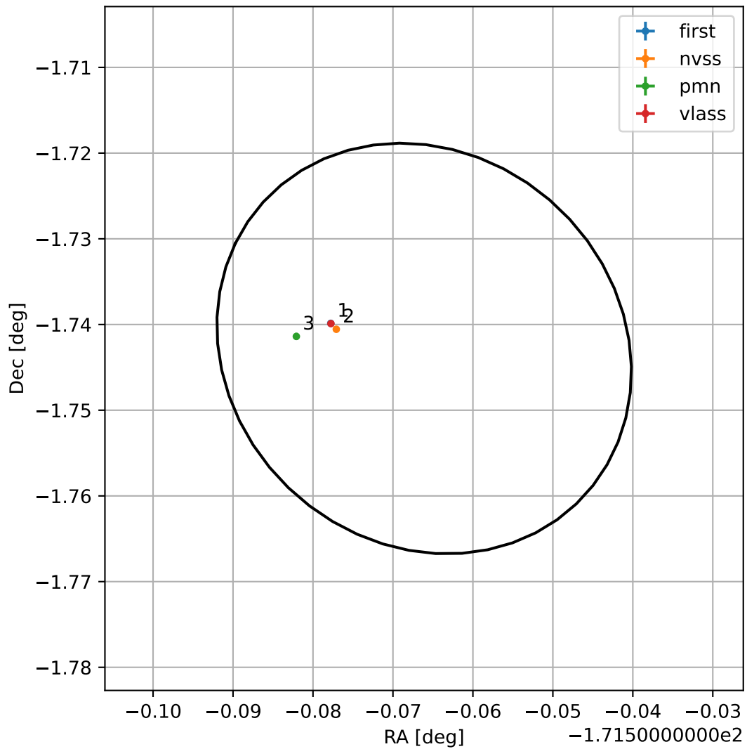
4FGL J1233.7-0144
