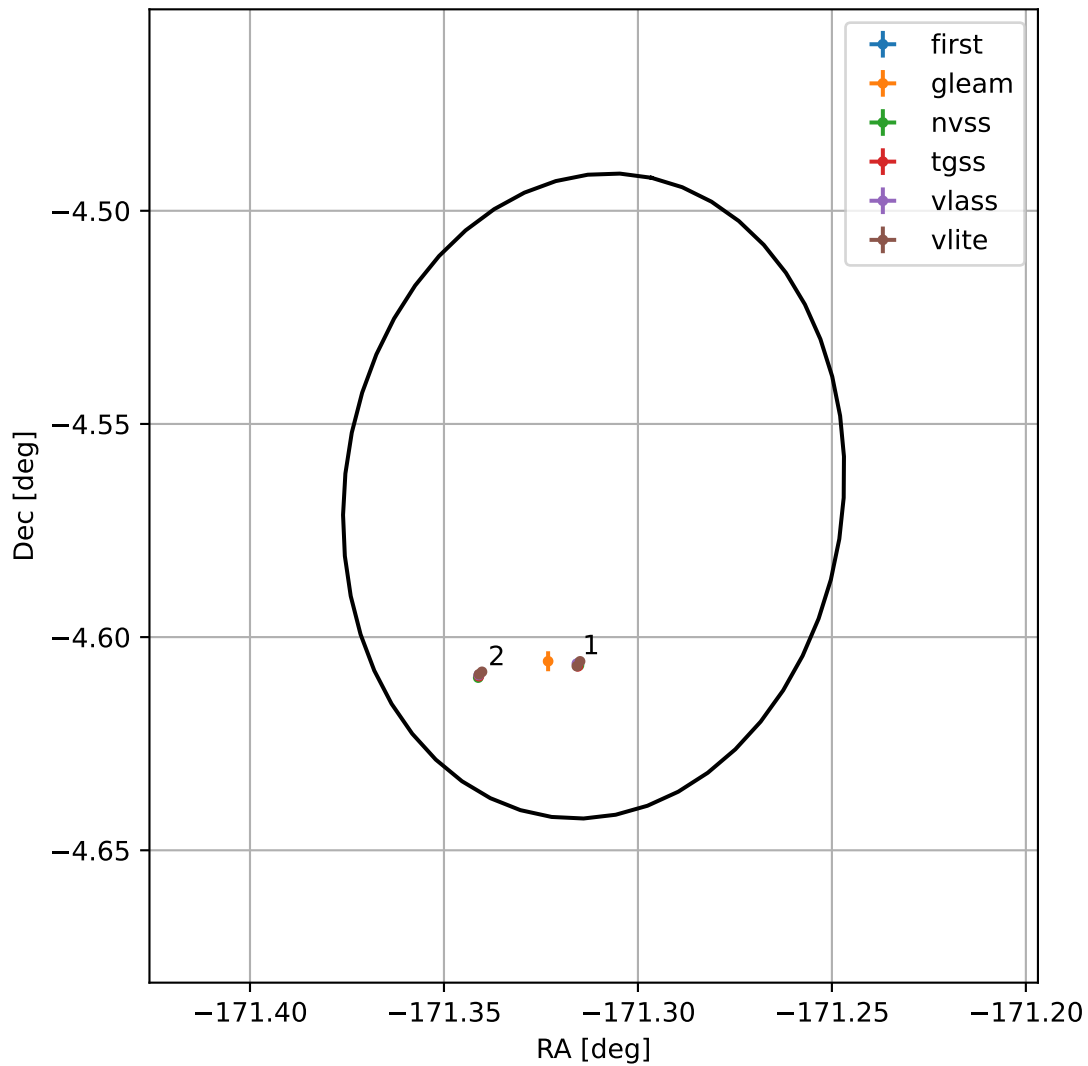
4FGL J1234.7-0434
