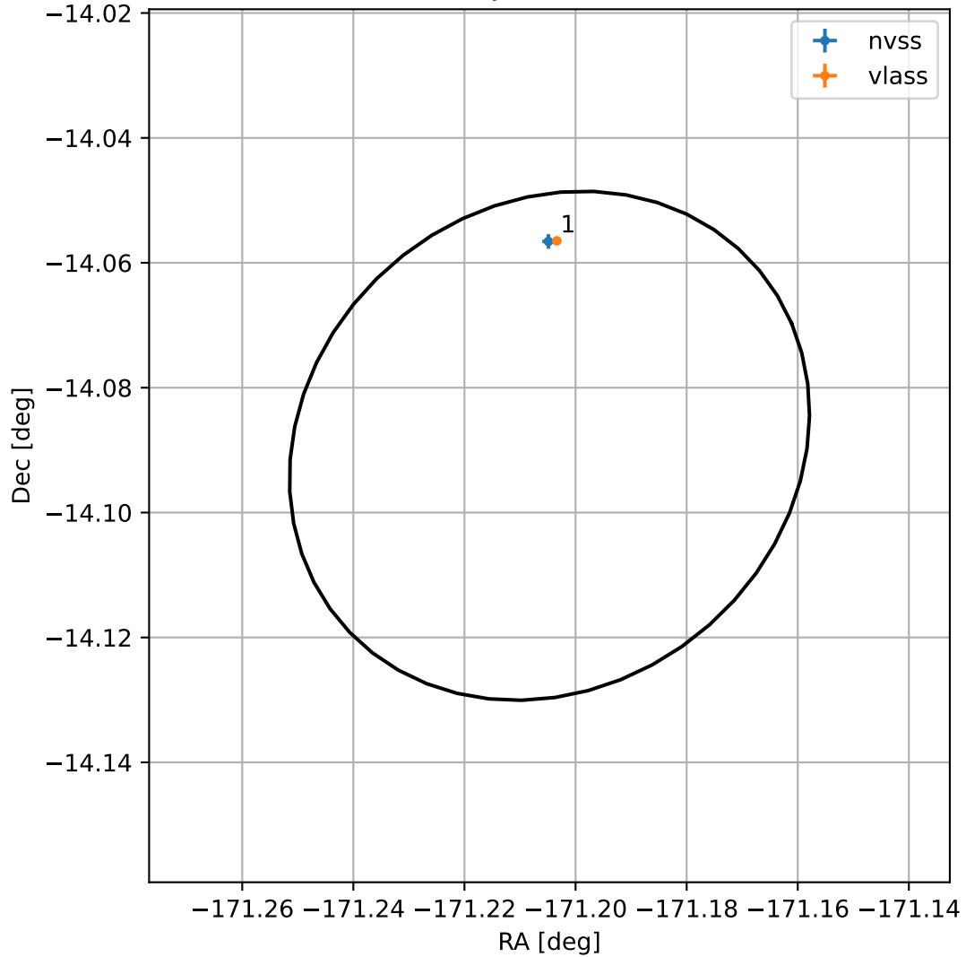
4FGL J1235.1-1405
