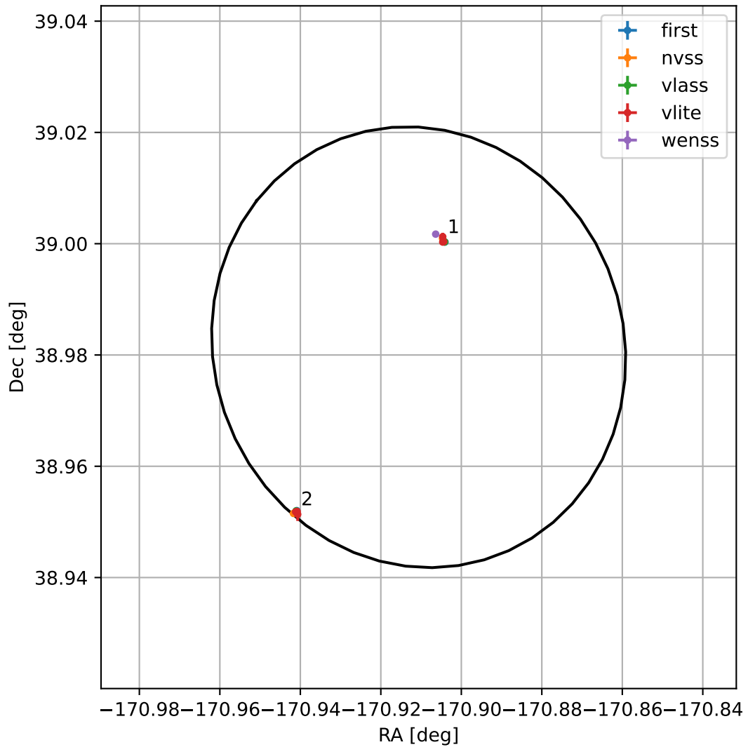
4FGL J1236.3+3858
