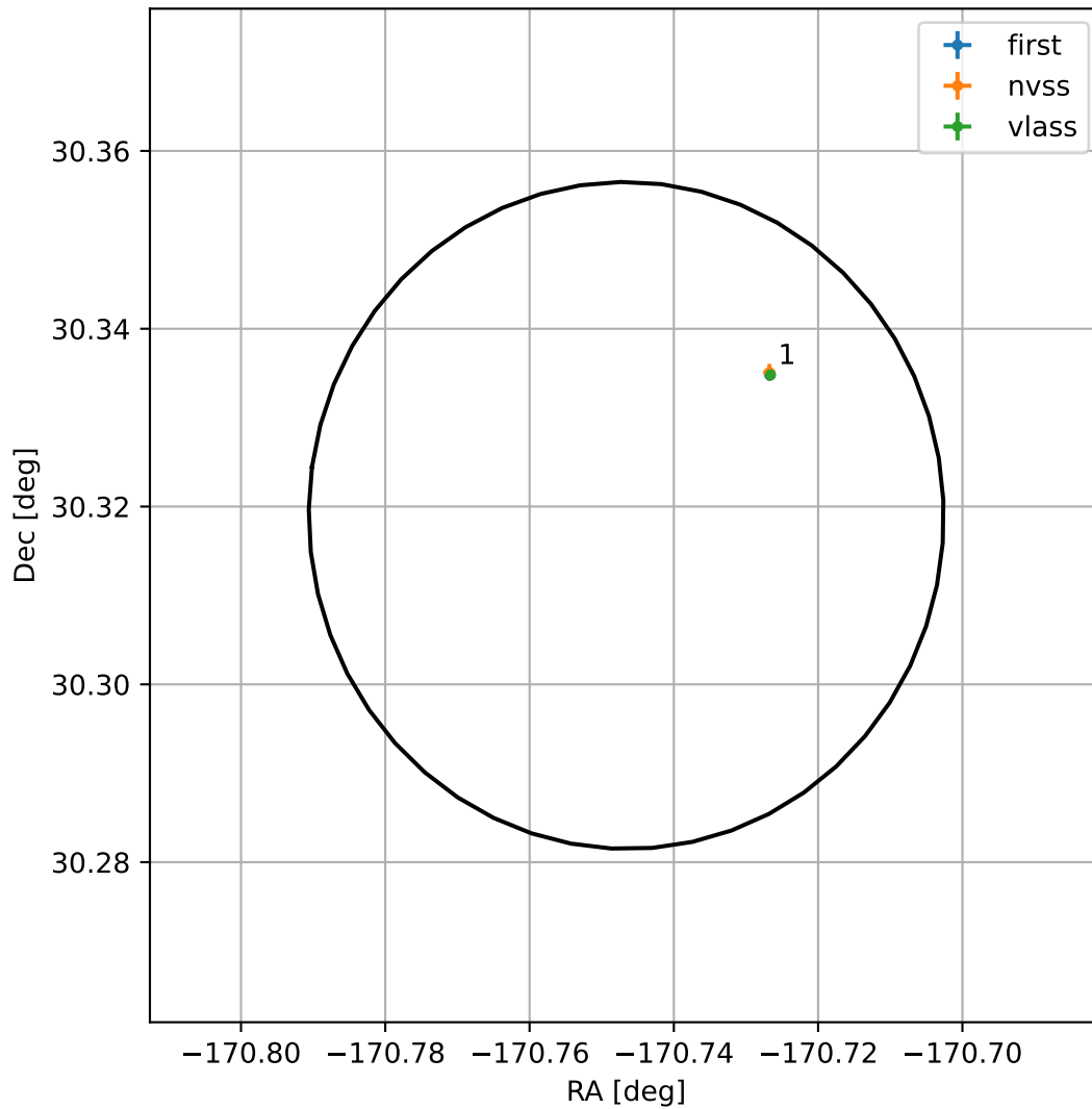
4FGL J1237.0+3019
