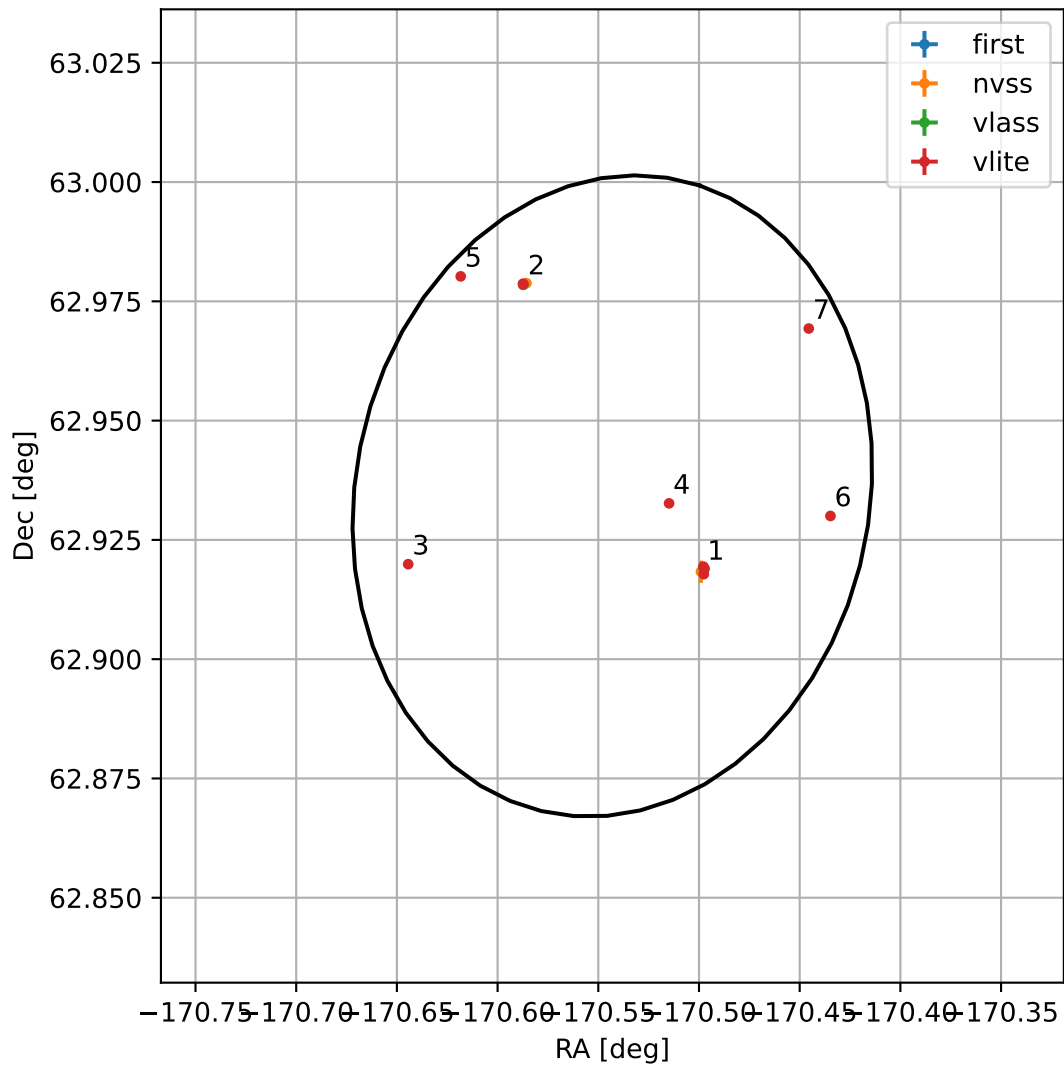
4FGL J1237.8+6256
