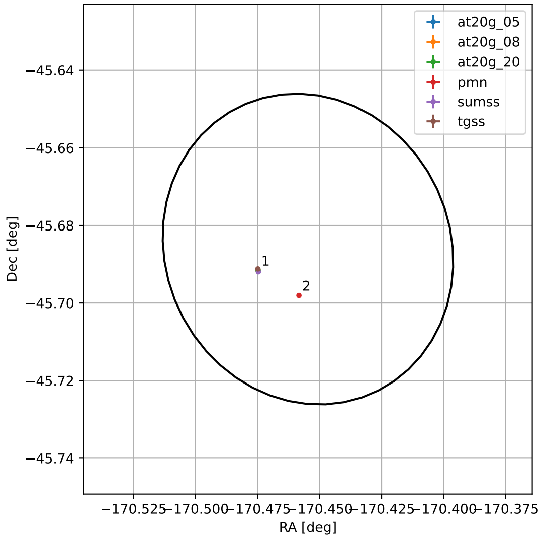
4FGL J1238.1-4541
