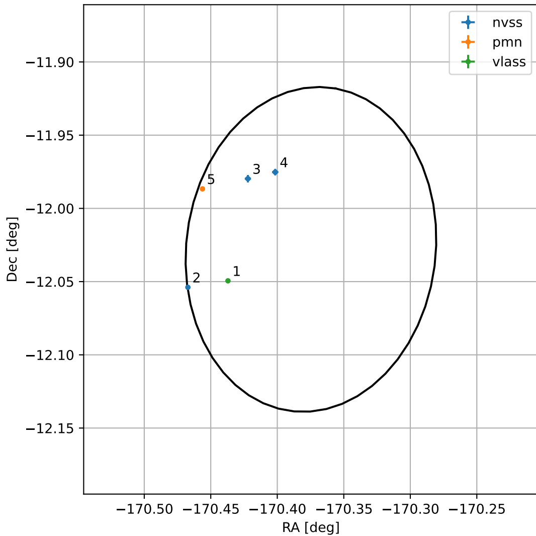
4FGL J1238.5-1201
