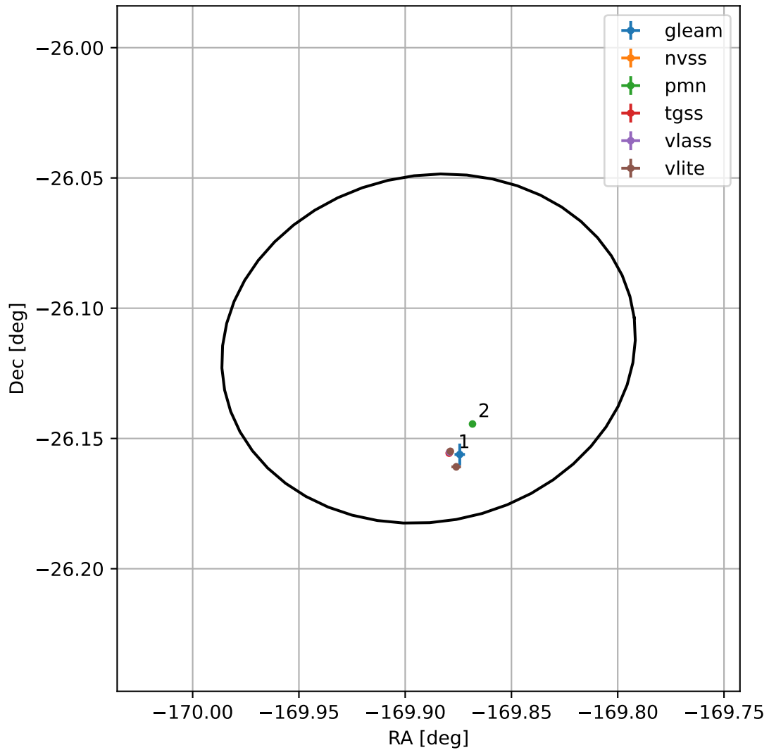
4FGL J1240.4-2606
