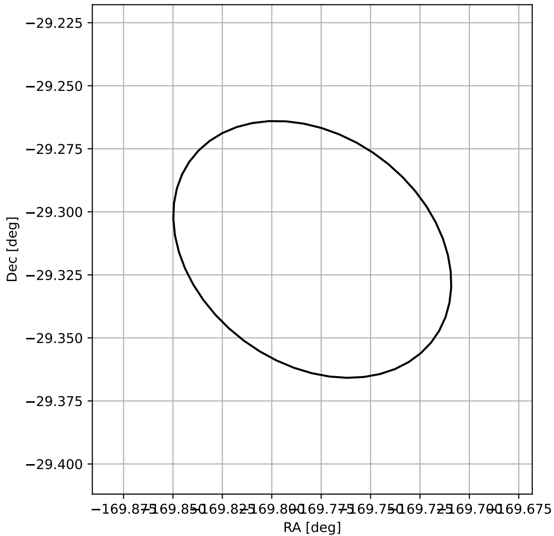
4FGL J1240.8-2918
