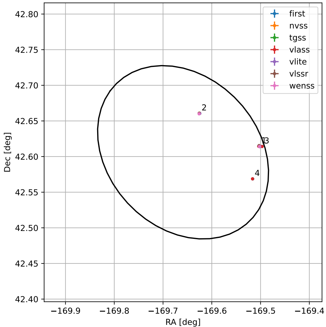
4FGL J1241.3+4236
