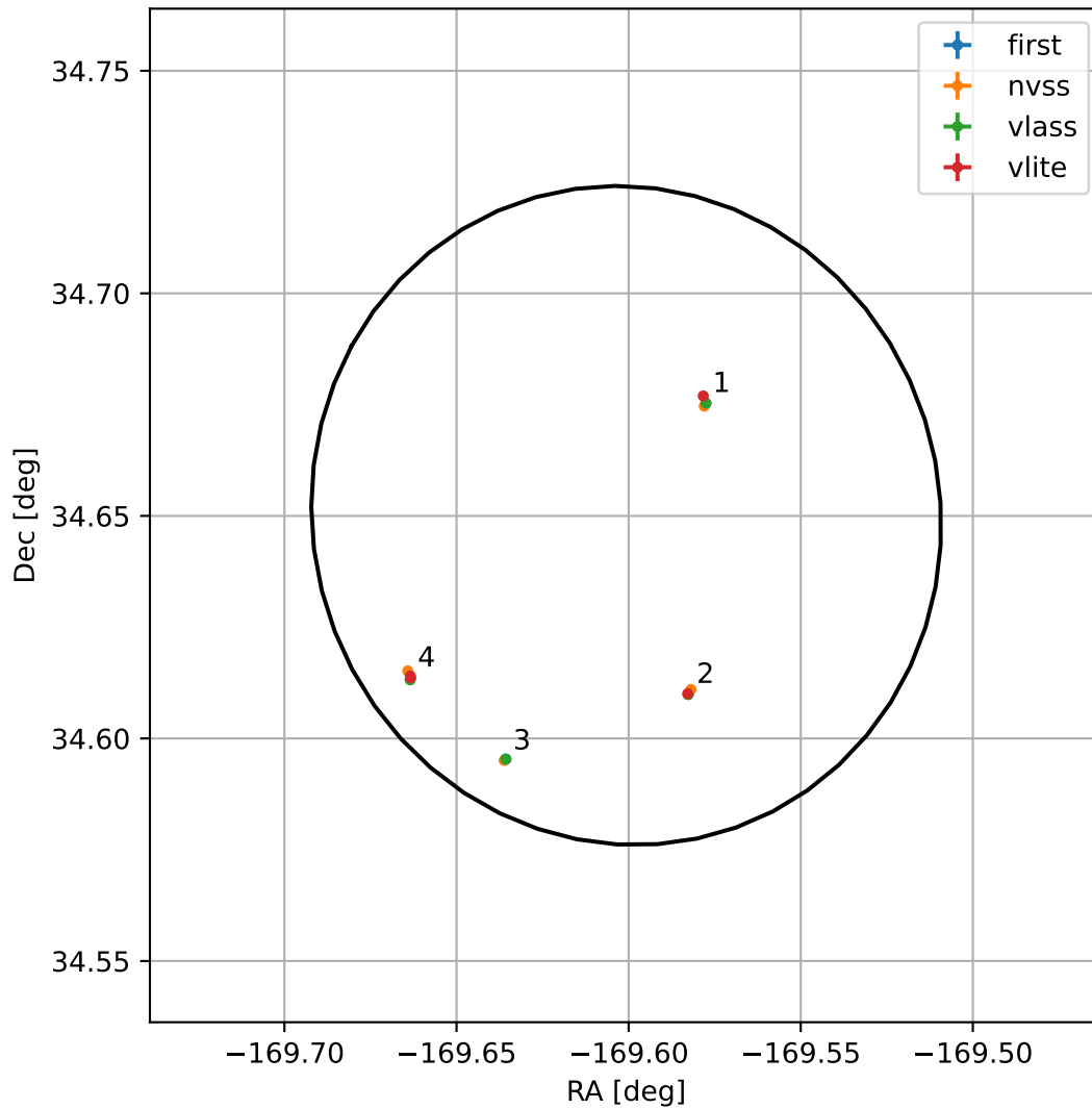
4FGL J1241.5+3439
