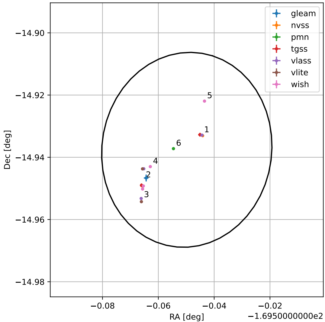
4FGL J1241.8-1456
