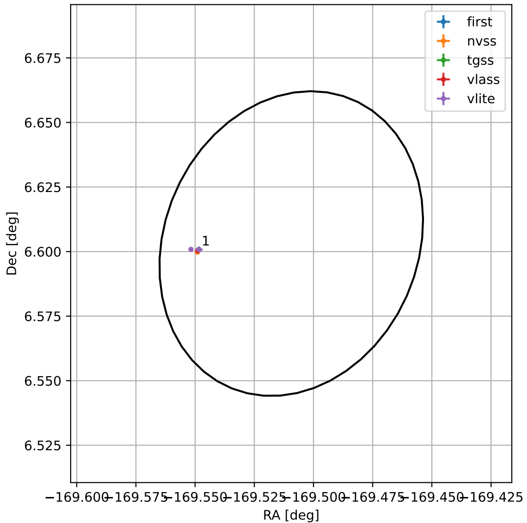
4FGL J1241.9+0636
