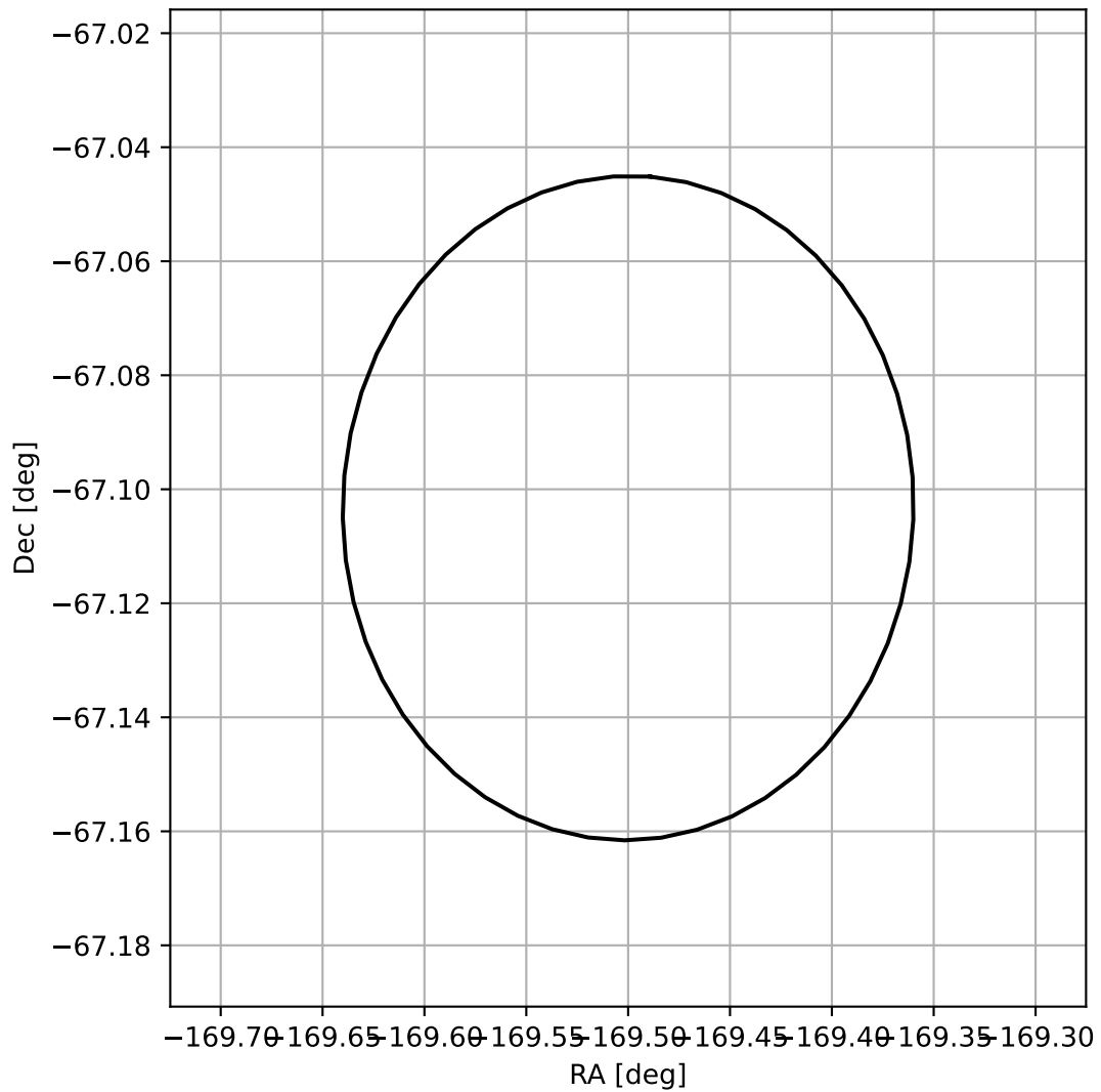
4FGL J1241.9-6706
