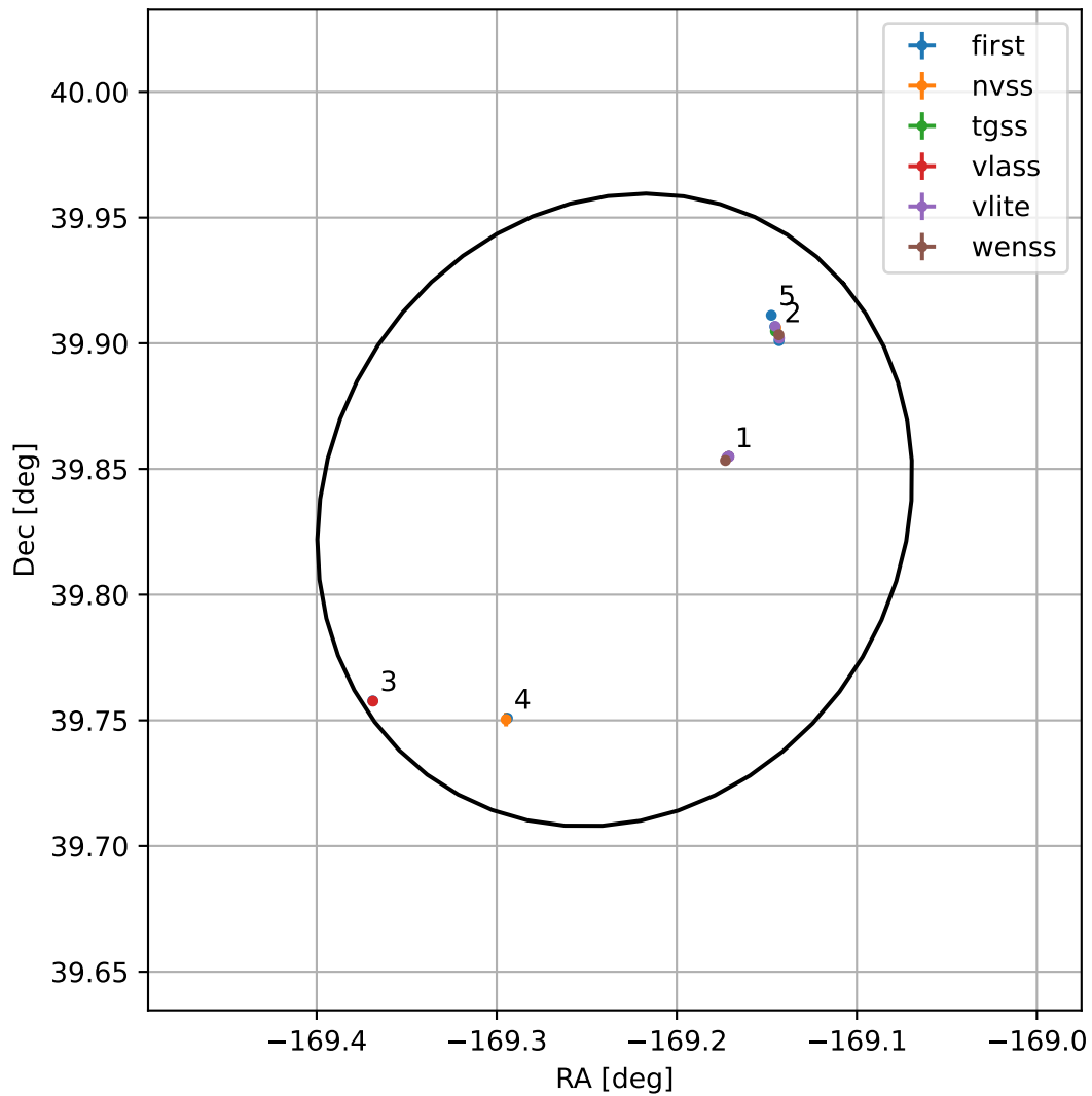
4FGL J1243.0+3950
