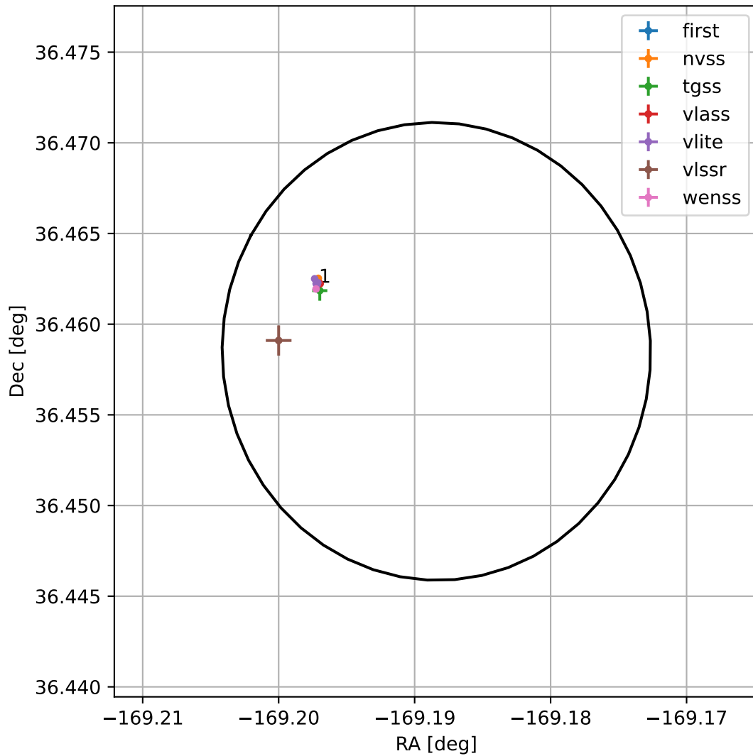
4FGL J1243.2+3627
