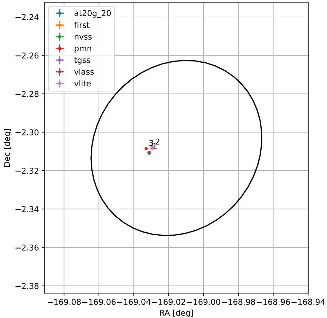
4FGL J1243.9-0218
