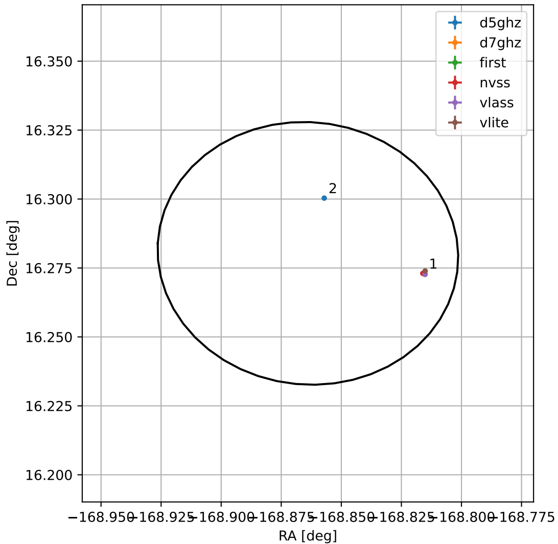
4FGL J1244.5+1616
