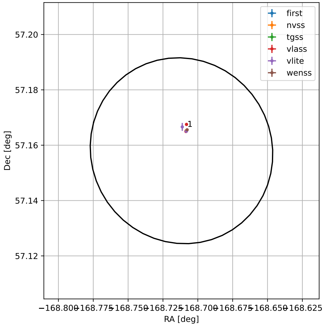
4FGL J1245.1+5709
