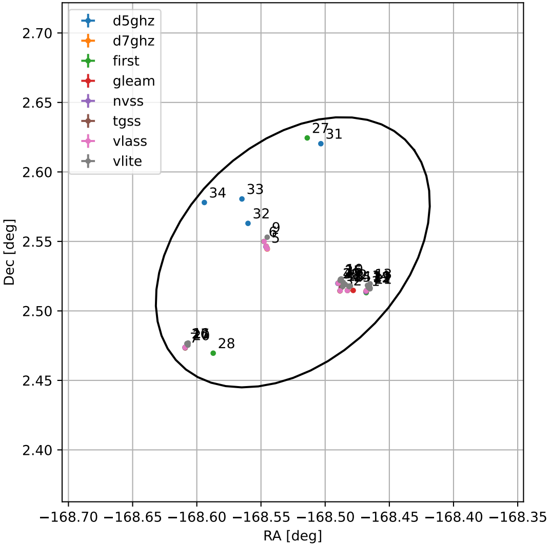
4FGL J1245.8+0232
