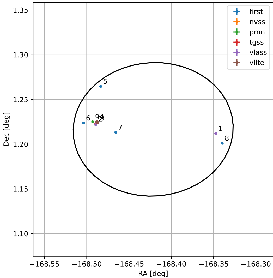
4FGL J1246.3+0112
